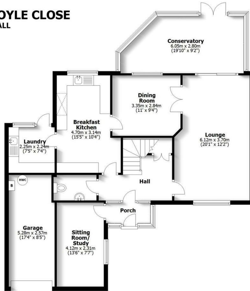
Ground Floor
